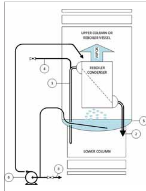
Figure 2: Example of film vaporizer. Credit: EPSIM Corp.
