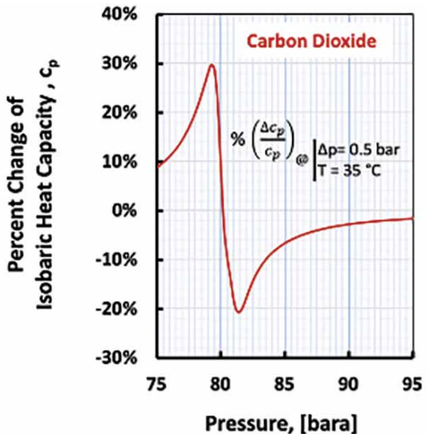
Figure 2: Sensitivity of isobaric heat capacity, c_p is examined for 0.5 bar change of pressure at a constant temperature of 35 °C across a range of pressures above the critical point of pure CO 2 [3] . Credit: Matt Taher, P.E.
